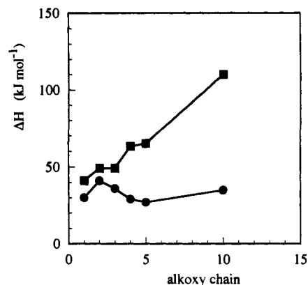
Figure 6. Plots of \Delta H and \Delta H_f versus the alkoxy chain of 2R' in 1-butanol; \Delta H was obtained from T_{gel} ( \blacksquare ), and \Delta H_f (melting energy) was obtained from DSC ( \bullet ).
