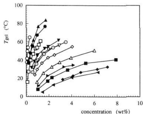
Figure 3. Plots of T_{gel} versus [2Pr'] : methanol ( \square ), 1-propanol ( \nabla ), 1-butanol ( \diamond ), 1-hexanol ( \Delta ), 2-propanol ( \blacktriangledown ), acetone ( \blacksquare ), n -hexane ( \blacklozenge ), acetic acid ( \odot ), methyl acetate ( \blacktriangleleft ), DMF ( \blacktriangleright ), dimethylpolysiloxane ( \bullet ), and cyclomethicone ( \blacktriangle ).
