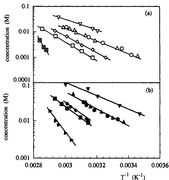
Figure 5. Plots of \log [2R'] versus T_{gel}^{-1} : (a) 2Me' in ethanol ( \nabla ), 2Et' in ethanol ( \circ ), 2Pr' in ethanol ( \Delta ), 2Bu' in ethanol ( \diamond ), 2Pent' in ethanol ( \square ), and 2Dec' in ethanol ( \square ); (b) 2Me' in 1-butanol ( \nabla ), 2Et' in 1-butanol ( \circ ), 2Pr' in 1-butanol ( \Delta ), 2Bu' in 1-butanol ( \diamond ), 2Pent' in 1-butanol ( \square ), and 2Dec' in 1-butanol ( \square ).
