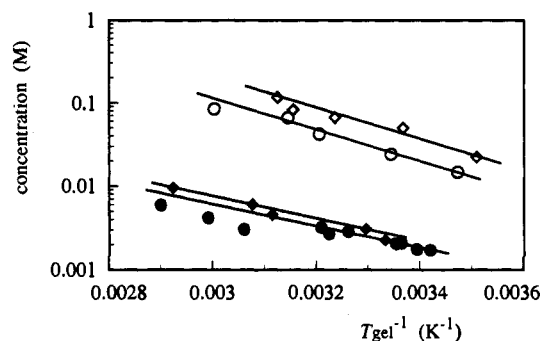
Figure 7. Plots of \log [2Me] and \log [2Me'] versus T_{gel}^{-1} : 2Me in 1-butanol ( \bullet ), 2Me in 1-octanol ( \blacklozenge ), 2Me' in 1-butanol ( \circ ), and 2Me' in 1-octanol ( \diamond ).
