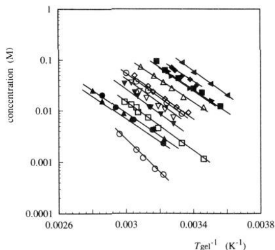
Figure 4. Plots of \log [2Pr'] versus T_{gel}^{-1} ; the symbols indicate the same solvents as those in Figure 3.
