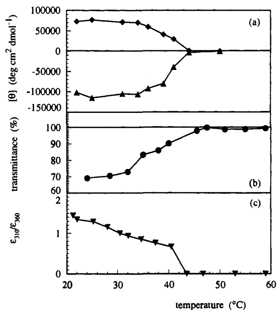
Figure 9. Temperature dependence of (a) maximum ( \blacklozenge ) and minimum ( \blacktriangle ) intensities of the CD spectra, (b) the transmittance at 800 nm, and (c) the ratio of the absorption spectral maxima at 310–360 nm for 2Me' (0.2 wt %) in 1-butanol.
